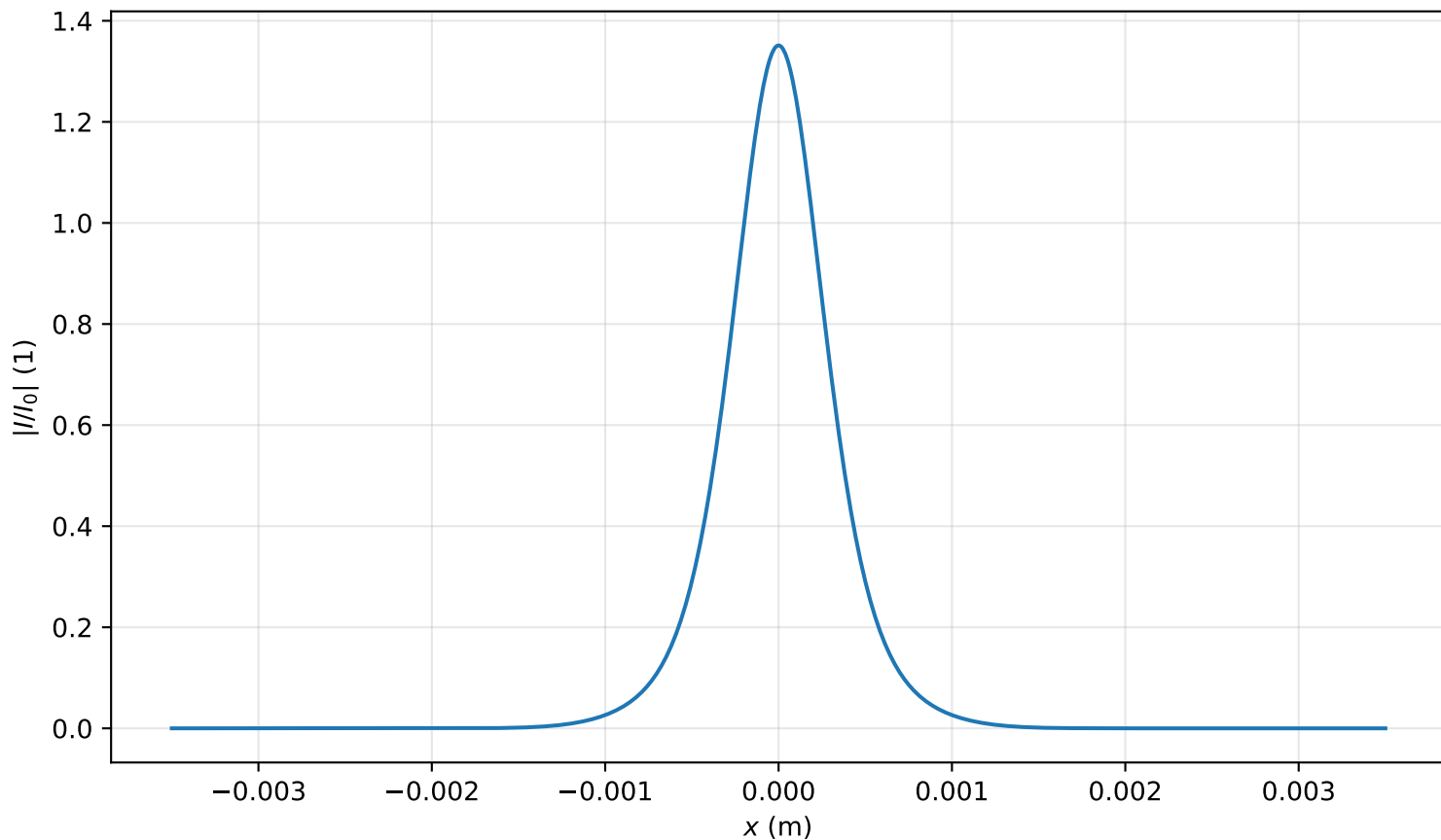
Intensity profile I(x, y = 0, z = 1.353m)/I_0 , P_{in}=0.8P_{cr} , artificial time
